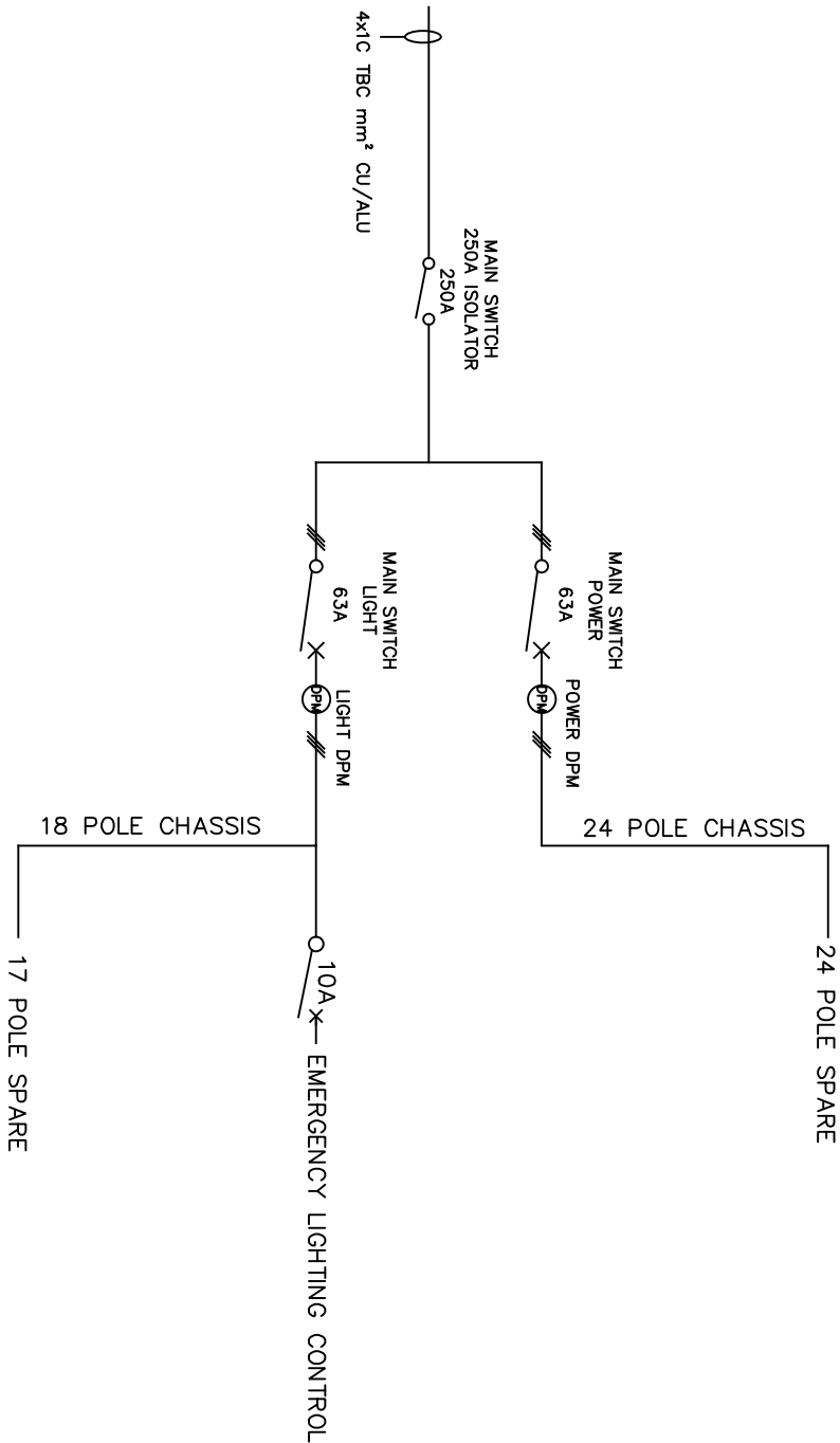
SINGLE LINE DIAGRAM
