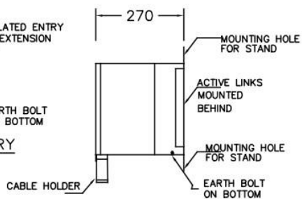
SIDE VIEW LID CLOSE
