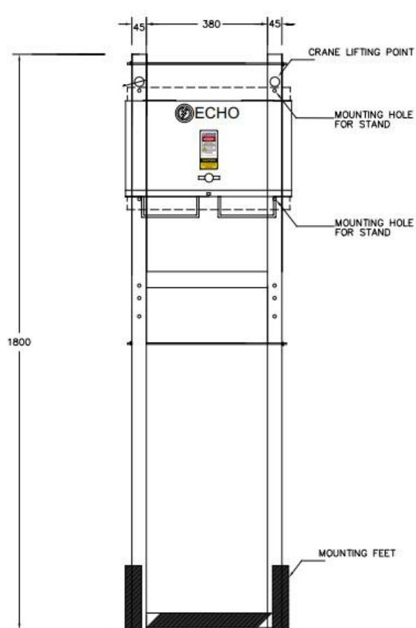
FRONT VIEW 1PH TEMP BOARD FITTED ON STAND
