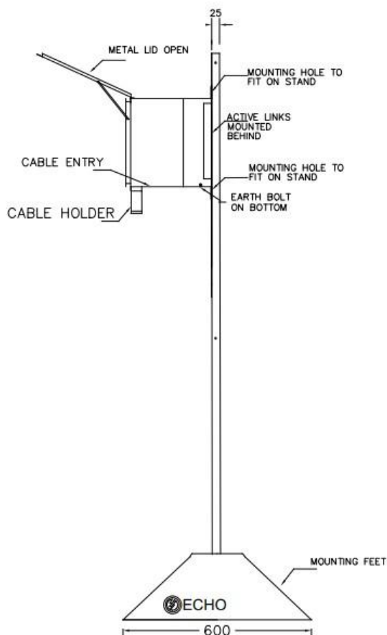
SIDE VIEW 1PH TEMP BOARD FITTED ON STAND
