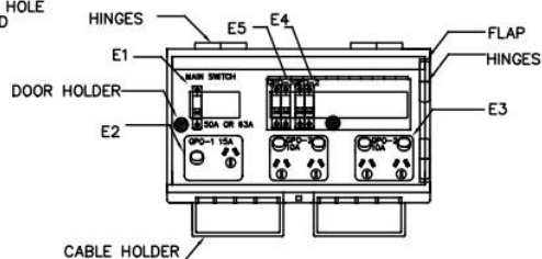
DOOR OPEN VIEW
