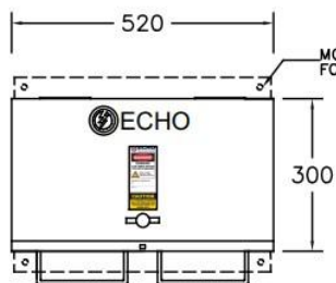
DOOR CLOSED VIEW
