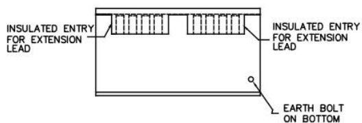
BOTTOM VIEW FOR CABLE ENTRY
