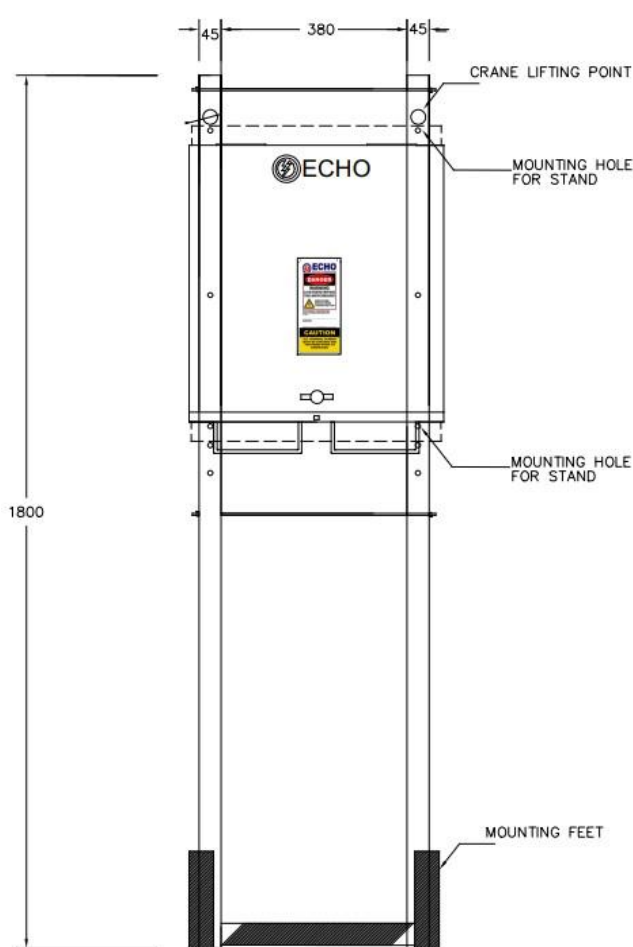
FRONT VIEW 3PH TEMP BOARD FITTED ON STAND
