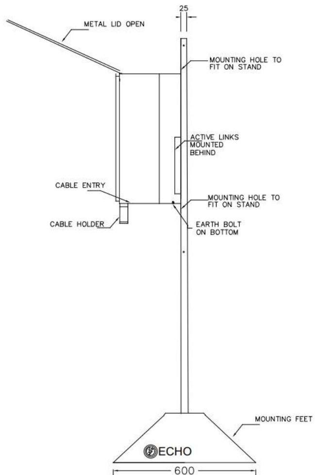
SIDE VIEW 3PH TEMP BOARD FITTED ON STAND
